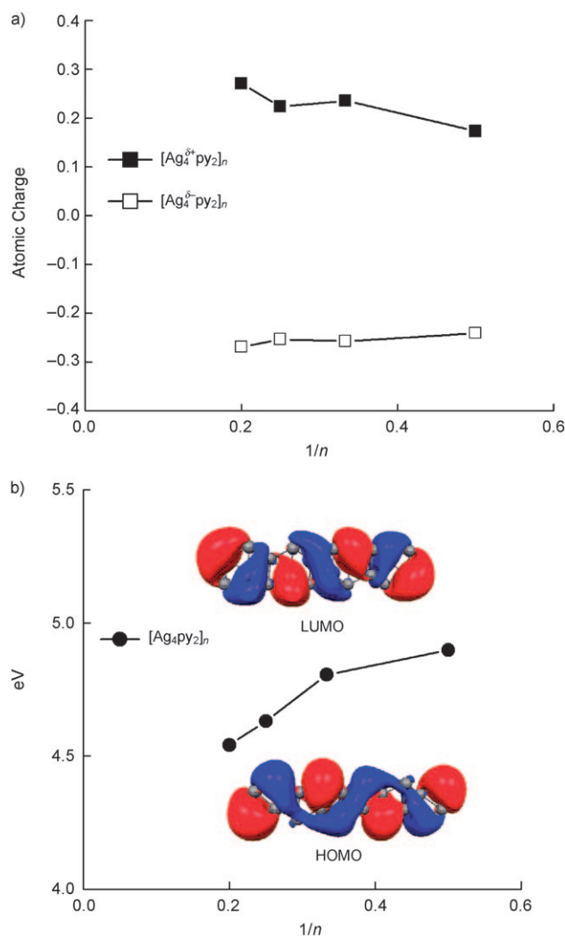
Figure 3. Theoretical calculations on [Ag_4py_2]_n ( 1 ). a) The calculated atomic charges for the Ag atoms as a function of model cluster size ( n=2-5 ). The limiting values are obtained by extrapolation to 1/n=0 . b) The calculated HOMO-LUMO gaps as a function of model cluster size ( n=2-5 ). The limiting values are obtained by extrapolation to 1/n=0 .
